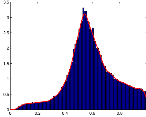
Figure 3: Posterior distribution of the learning parameter \beta with kernel density estimation of the likelihood and MCMC sampling. 400,000 simulations of 1,500 trading days each are performed. 1,500 pseudo-true trading days are assumed to be observed. The pseudo-true value is \beta = 0.55 .
