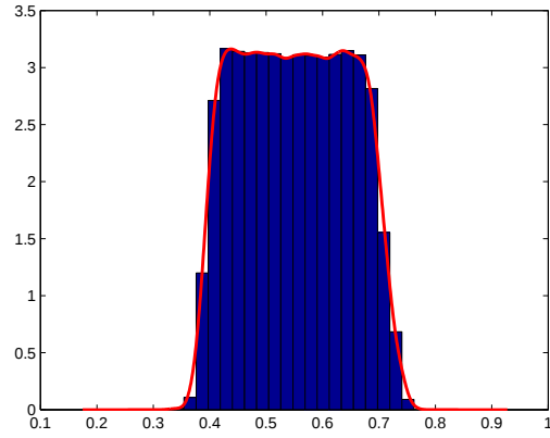
Figure 7: Posterior distribution of the learning parameter \beta with likelihood-free ABC estimation and rejection sampling. 400,000 simulations of 1,500 periods each are performed. 1,500 pseudo-true periods are assumed to be observed. Different values of the tolerance threshold are considered (the variance of price, used as summary statistics, ranges approximately from 0 to 5). The pseudo-true value is \beta = 0.55 .
